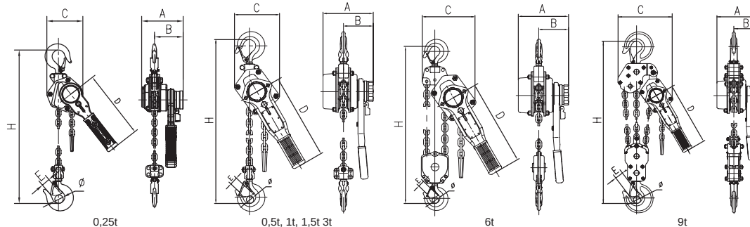
Fig. 1 Dimensioned sketch
